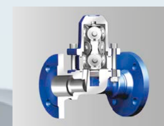
For higher flow rate CONA® M 616 diaphragm multi-capsule thermostatic steam trap (4, 6 or 10 capsules)
