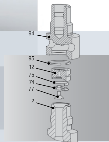
RO Series O-Ring Soft Seat Design
