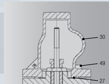
Bolted Gastight Cap
