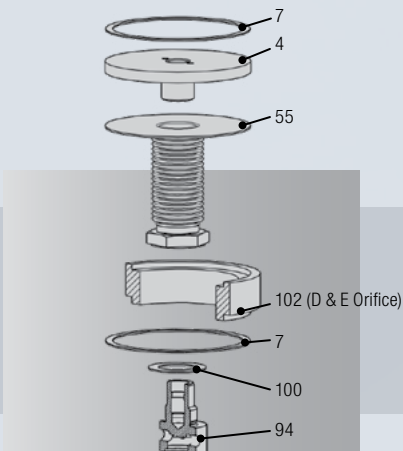
REYCO® RB & RBO Balanced Bellows Design
