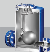
Mechanical Condensate Pump CONLIFT®
