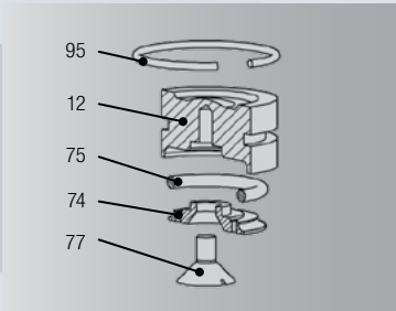
REYCO® RO & RBO O-Ring Soft Seat Design
