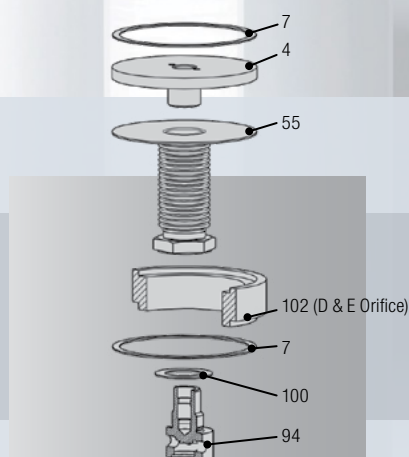
RB Series Balanced Bellows Design
